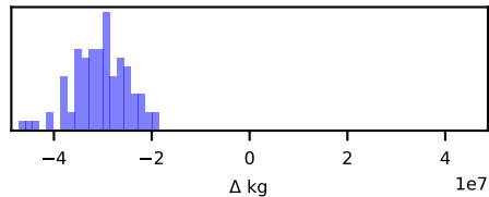
(i) Difference, one-layer
