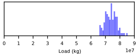
(g) With Tr, one-layer
