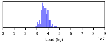
(e) Without Tr, two-layer
