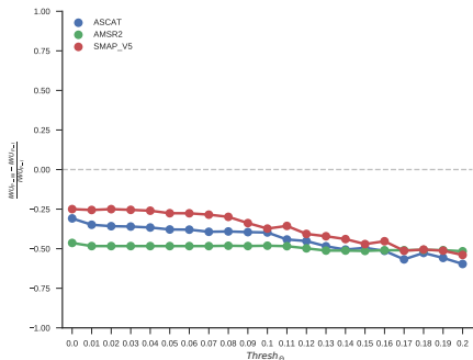
(c) Nebraska plains
