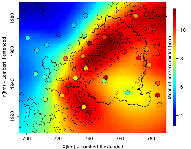
Mean of nonzero rainfall in S2 WP2
