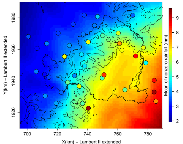
Mean of nonzero rainfall in S2 WP3
