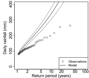
lnorm-(2,3)
