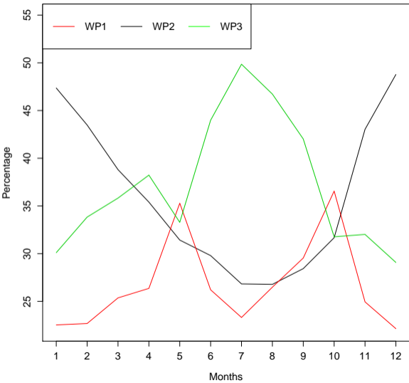
(a) Monthly percentage of WP occurrence
