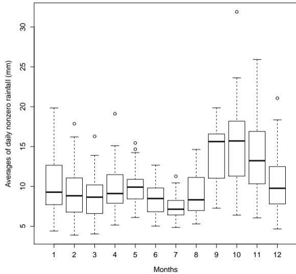
(b) Monthly averages of daily nonzero rainfall
