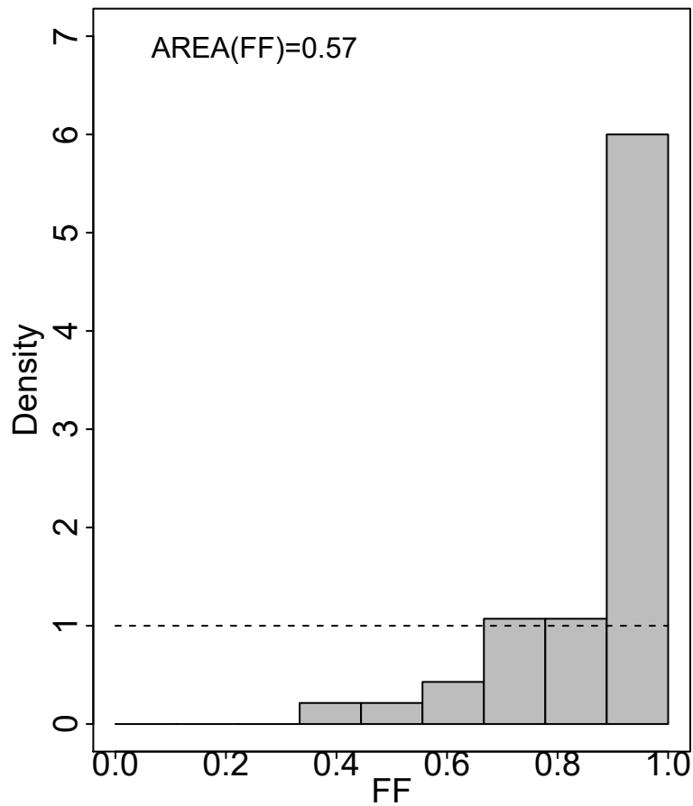
(c) Histogram of FF under G_2
