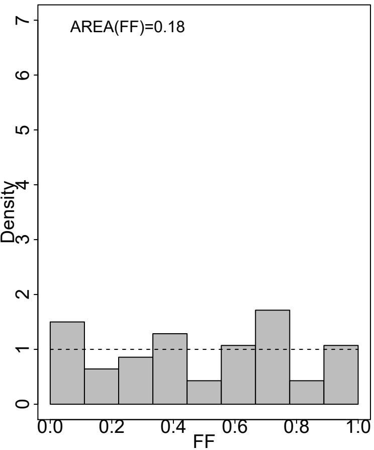
(a) Histogram of FF under G_0
