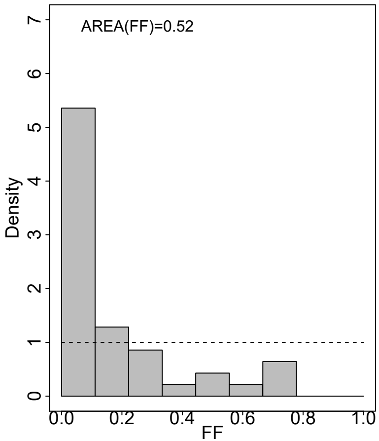
(b) Histogram of FF under G_1
