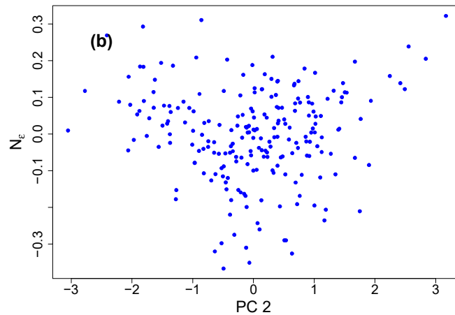
Residuals vs. PC 2
