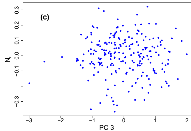
Residuals vs. PC 3
