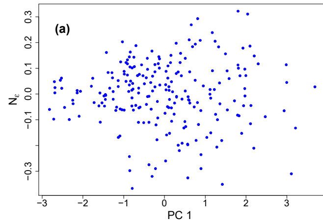
Residuals vs. PC 1
