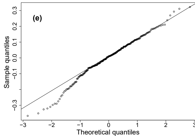
Normal Q-Q plot of residuals
