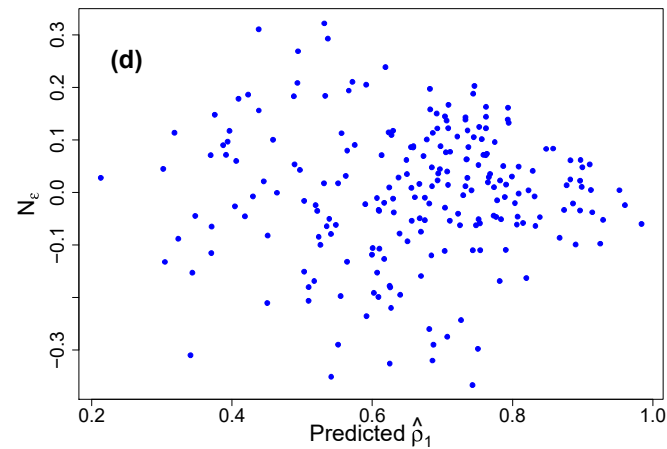
Residuals vs. predicted
