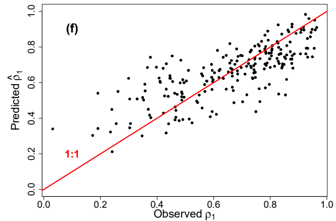
Predicted vs. observed
