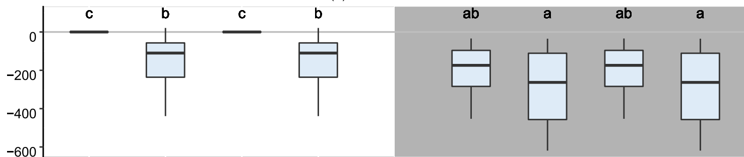
(c) Peak SWE: wind sheltered
