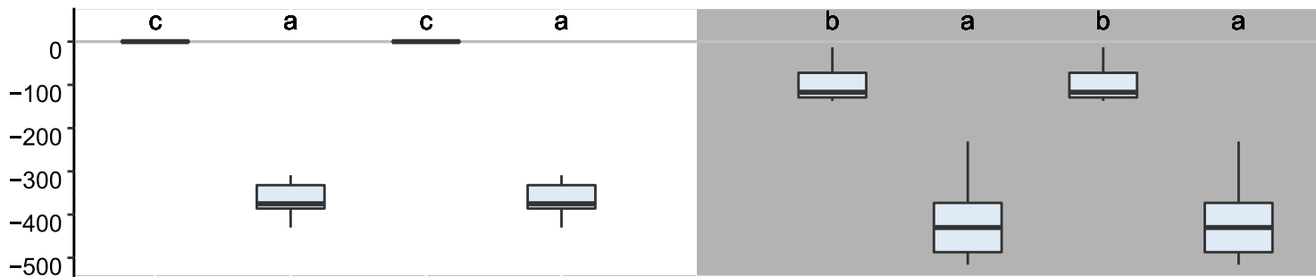
(e) Annual runoff
