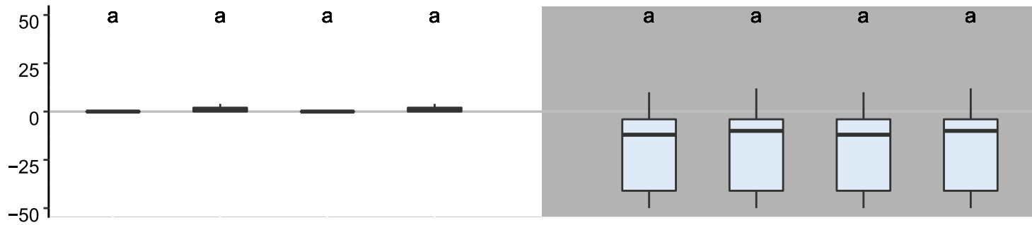
(b) Peak SWE: forest
