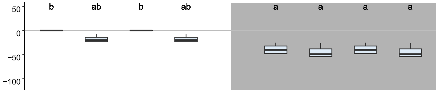
(c) Peak SWE: forest clearing
