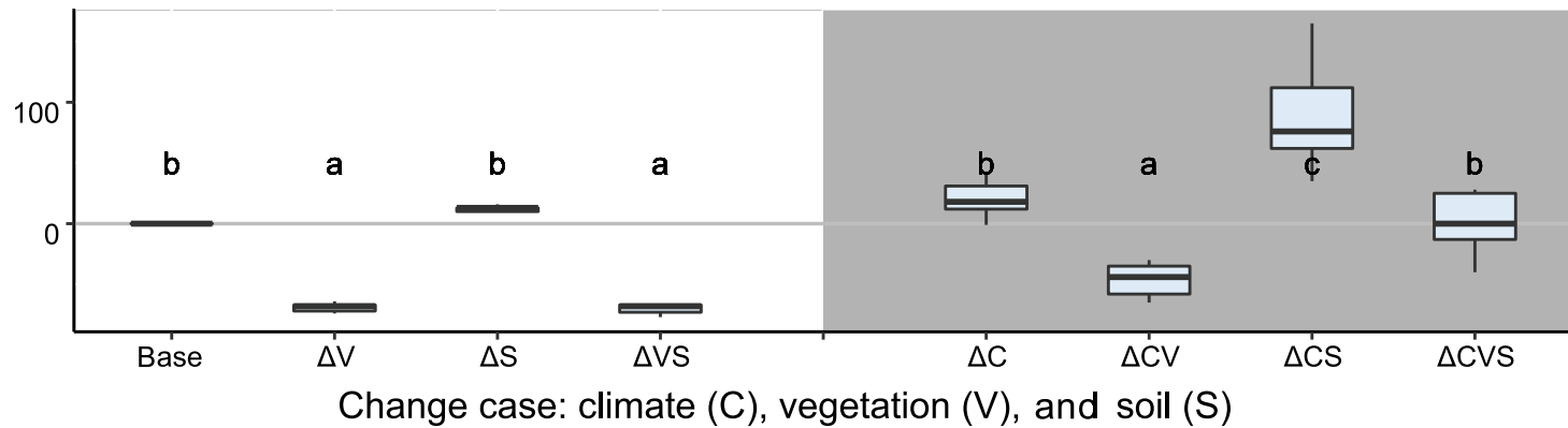
(e) Annual runoff
