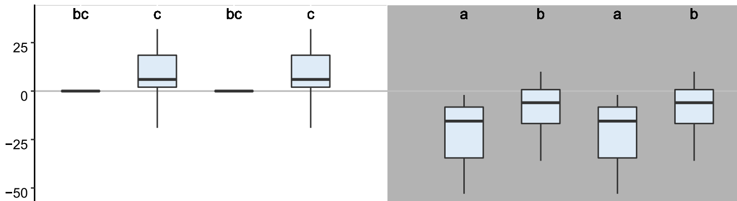
(b) Peak SWE: shrub tundra
