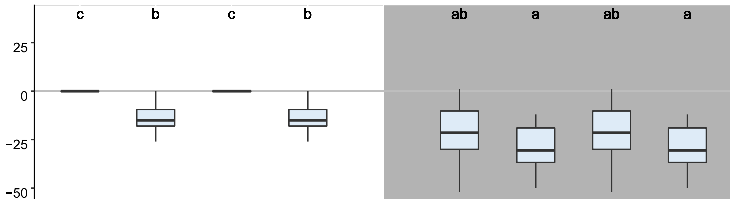
(c) Peak SWE: forest
