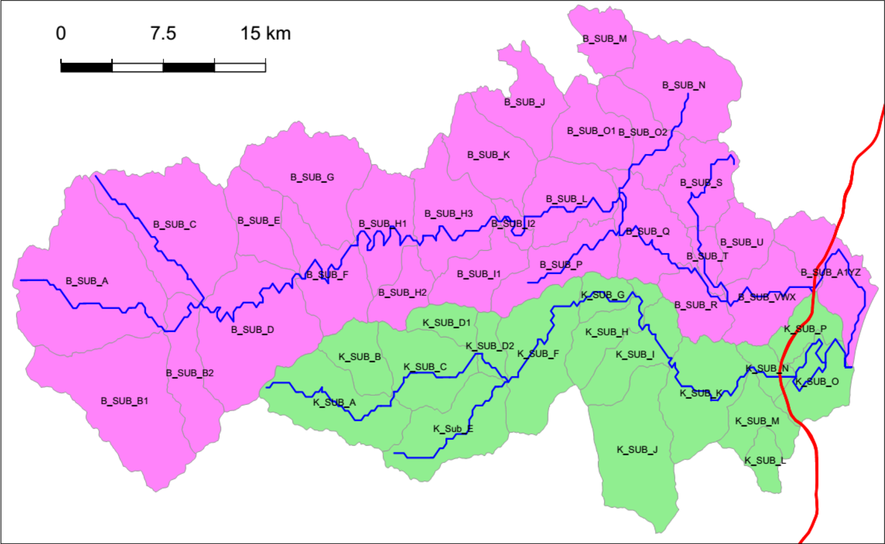
Fig. S3. Hydrological model layout for Bellinger catchment and Kalang River catchment. The blue lines are the river network, and the red line is the Pacific Highway upgrade project.
