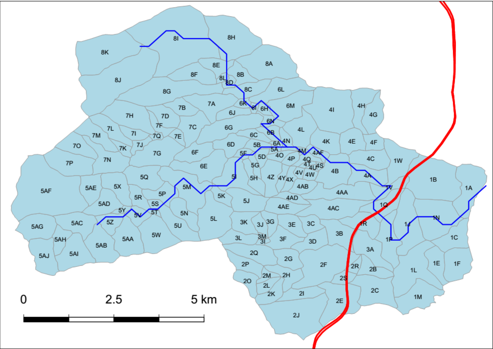
Fig. S5. Hydrological model layout for Deep Creek catchment. The blue lines are the river network, and the red line is the Pacific Highway upgrade project.
