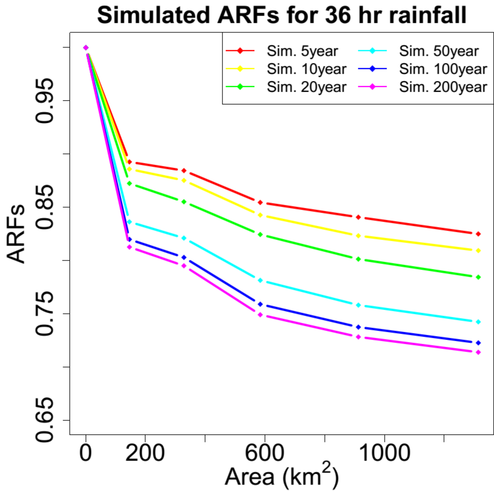
Fig. S1. Simulated ARFs for spatial rainfall of 36 hr duration for different return periods.
