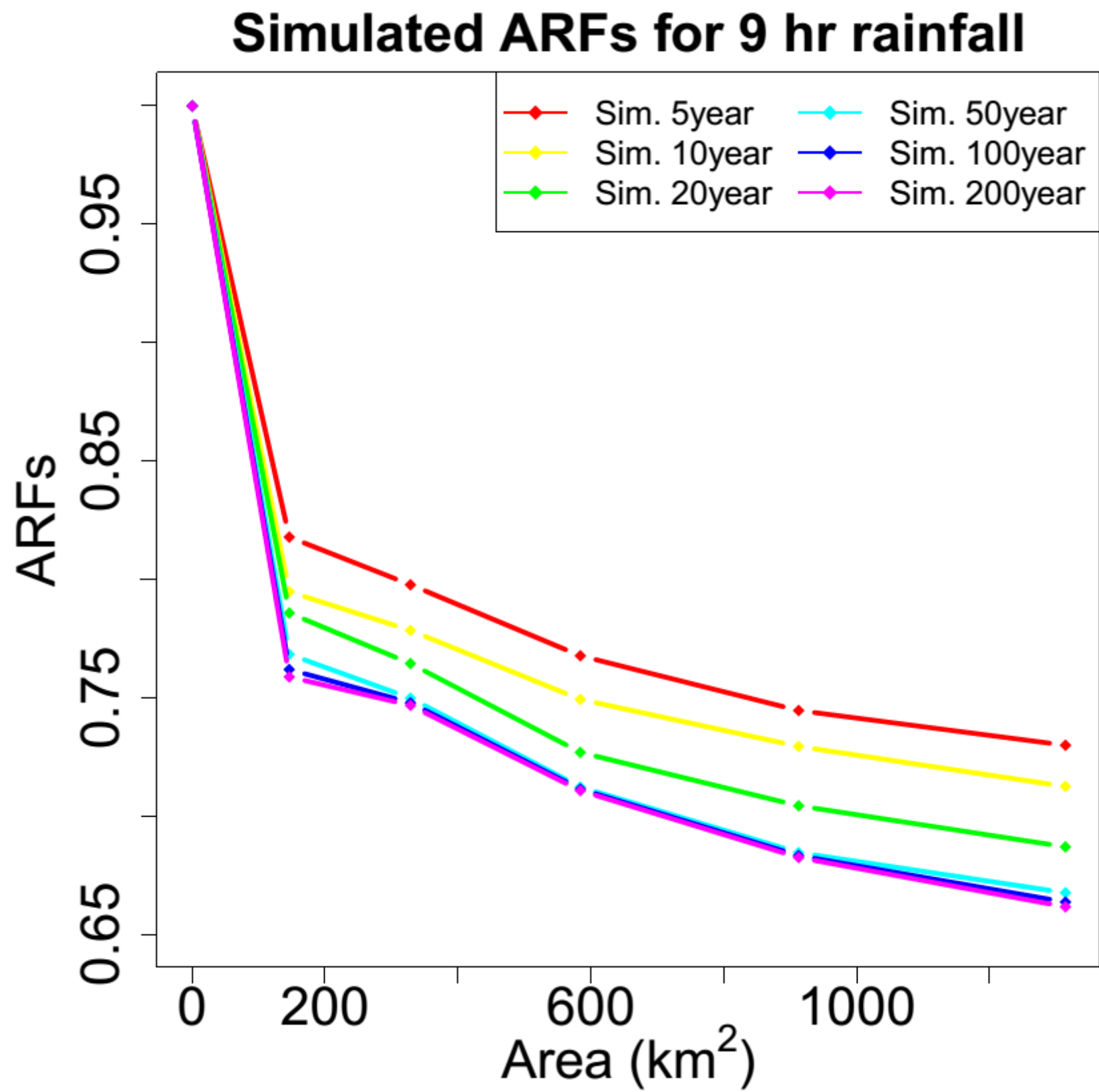
Fig. S2. Simulated ARFs for spatial rainfall of 9 hr duration for different return periods.
