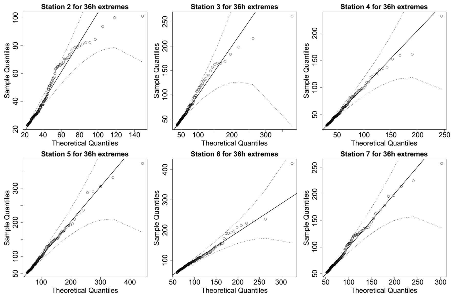
Fig. S6. QQ plots for the estimate of marginal distribution GPD for 36 hr rainfall extremes for rain gauges from 2 to 7. The solid diagonal line indicates a perfect fit, and the dotted lines indicate a 95% confidence interval.
