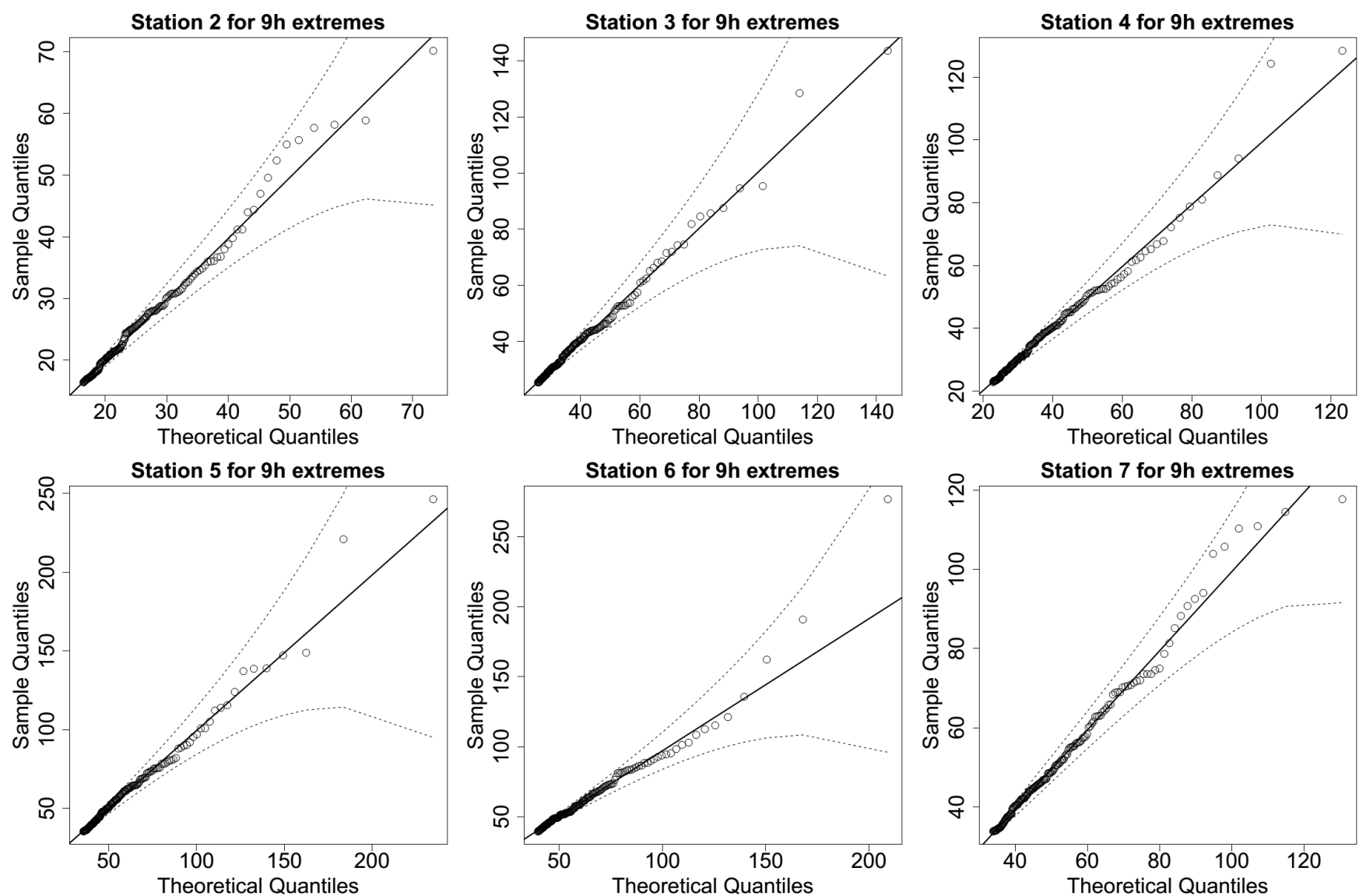
Fig. S7. QQ plots for the estimate of marginal distribution GPD for 9 hr rainfall extremes for rain gauges from 2 to 7. The solid diagonal line indicates a perfect fit, and the dotted lines indicate a 95% confidence interval.
