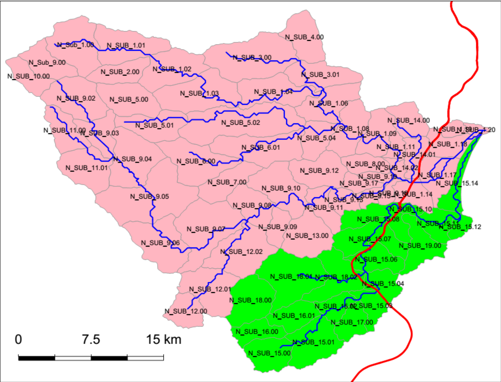
Fig. S4. Hydrological model layout for Nambucca (upper) catchment and Warrell Creek catchment. The blue lines are the river network, and the red line is the Pacific Highway upgrade project.
