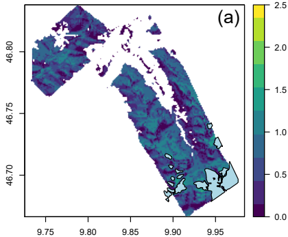
Prior median
