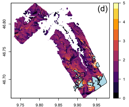
Prior 90Q
