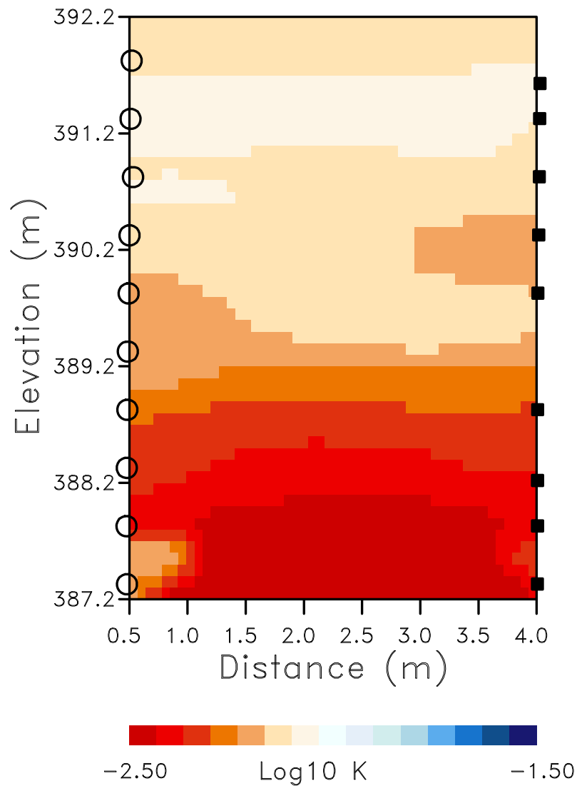
(a) Eikonal
