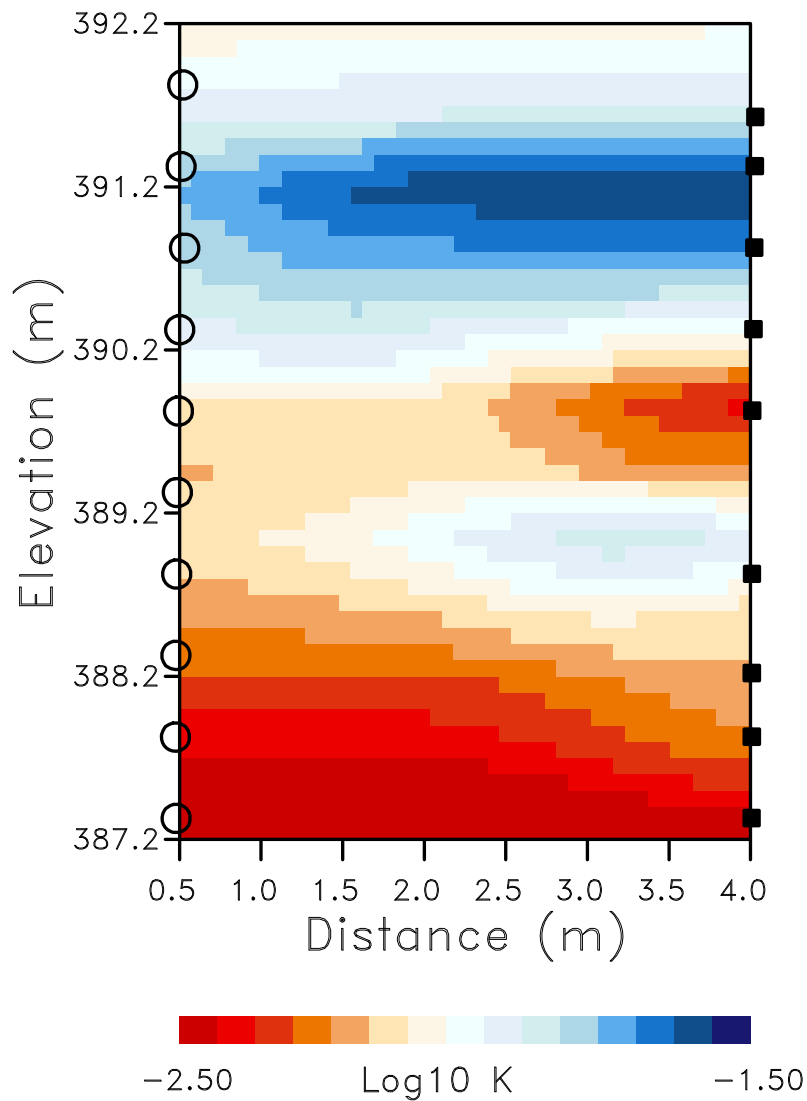
(b) Extended
