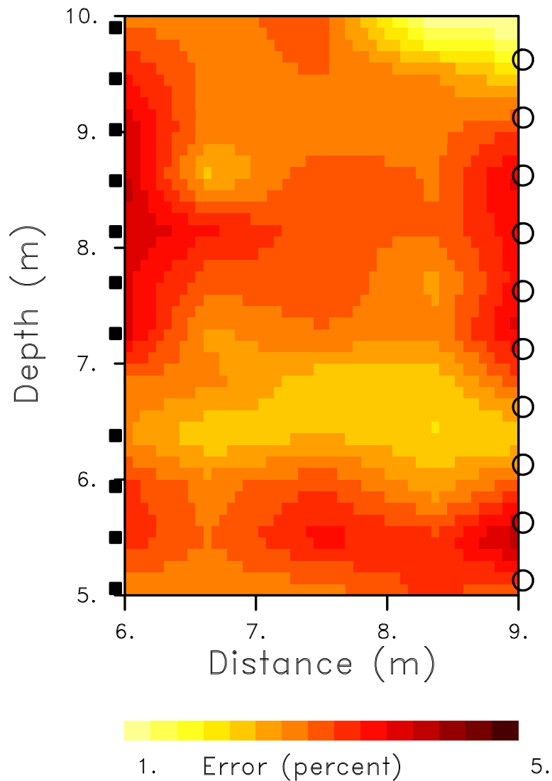
(b) Standard error
