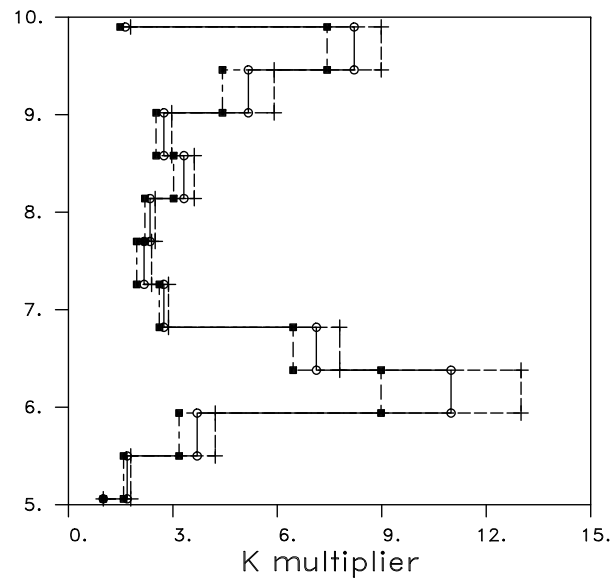
(c) Extended
