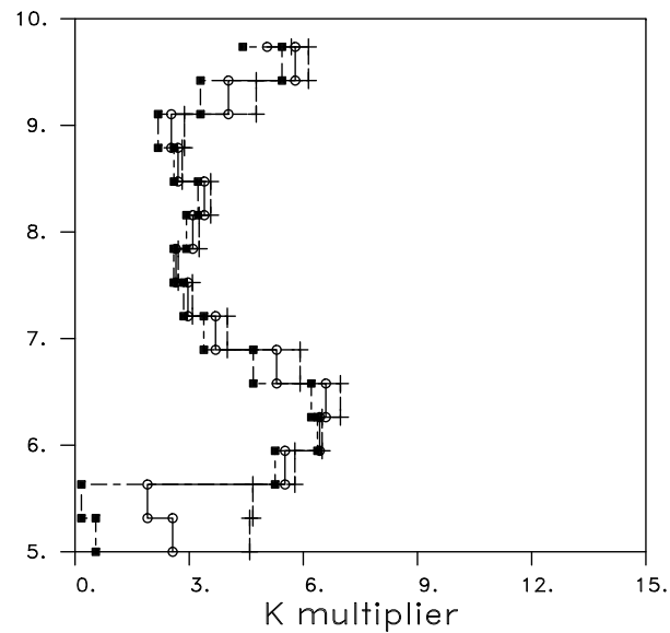
(b) Eikonal
