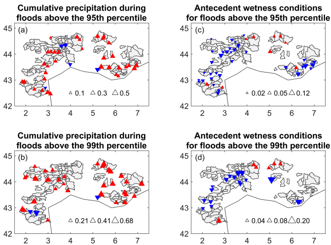
Figure 6. Significant trends at the 10 % level (Mann–Kendall test) in cumulative precipitation during flood events above the 95th and 99th percentile (a, b) and in the soil moisture initial conditions (c, d). Blue triangles indicate a decrease and red triangles an increase. The size of the triangles indicates the relative changes.
