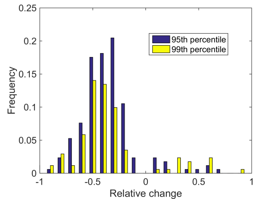
Figure 5. Histogram of the relative changes in the 95th and 99th percentiles estimated from the quantile regression models, with time as covariate (with a slope significantly different than zero at the 10 % level).
