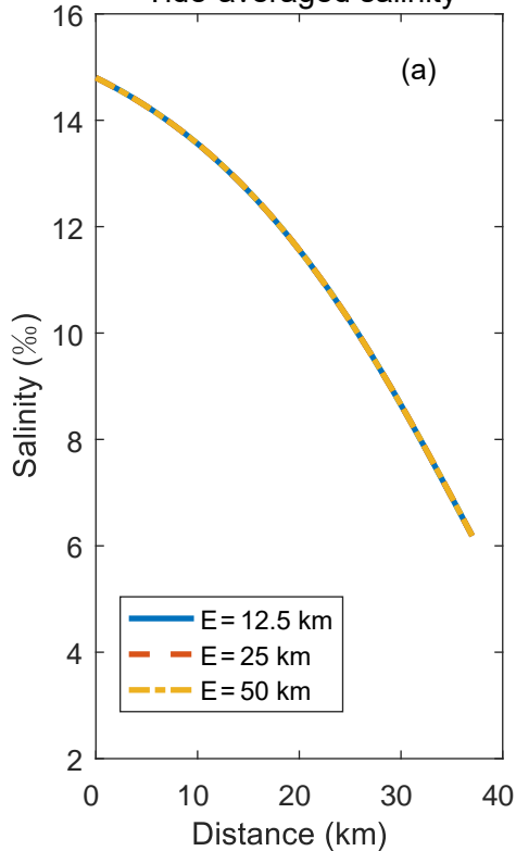
Tide-averaged salinity
