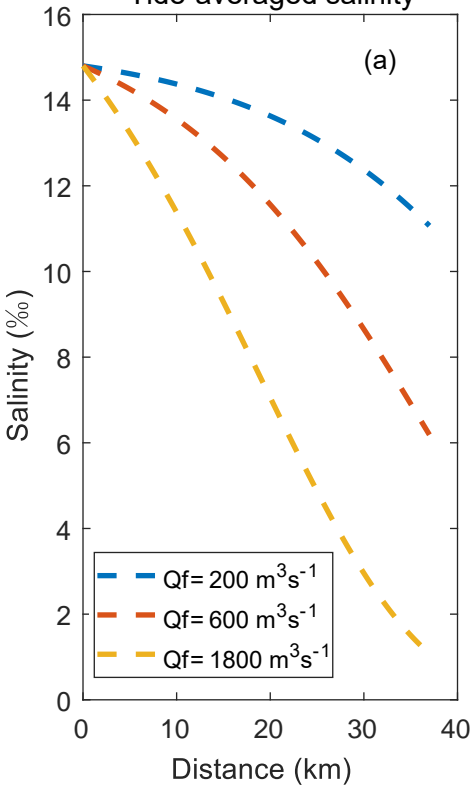
Tide-averaged salinity
