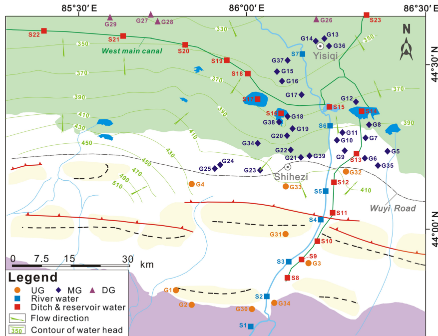
Figure 2. Water sampling sites and unconfined groundwater head contours (in metres) in the headwater catchments of Manas River. UG: upstream groundwater, MG: midstream groundwater, DG: downstream groundwater.
