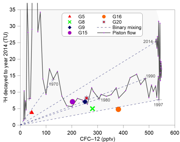
Figure 9. ^3\text{H} activity (TU) in Urumqi precipitation decayed to 2014 vs. CFC-12 in parts per trillion of volume (pptv) for Northern Hemisphere air. The “+” denotes selected calendar years. The solid lines correspond to the piston flow and the dashed lines show the binary mixing. The shaded region indicates concentrations that could arise due to mixing water of different ages.
