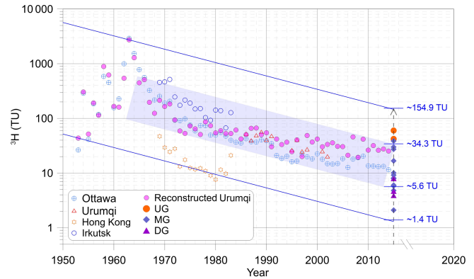
Figure 4. Tritium concentration (TU) of the upstream groundwater (UG), midstream groundwater (MG), and downstream groundwater (DG). Time series of tritium concentration in precipitation at Ottawa, Urumqi, Hong Kong, and Irkutsk were obtained by GNIP in IAEA ( https://www.iaea.org/ , last access: 4 December 2017). The blue solid lines and shaded field were drawn using the half-life (12.32 years) of tritium decayed to 2014.
