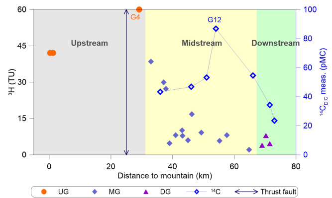
Figure 8. Distributions of ^3\text{H} and ^{14}\text{C} activities with distance to the mountain. The shaded regions indicate the upstream, midstream, and downstream of Manas River.
