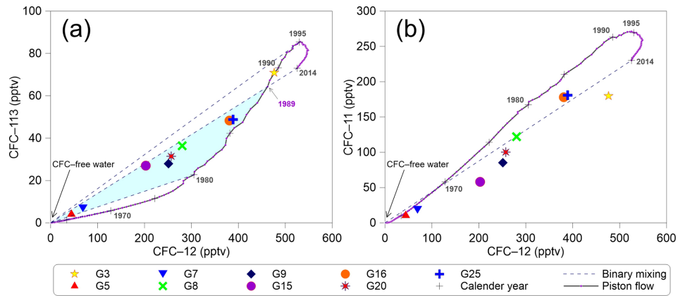
Figure 7. Plots showing relationships of (a) CFC-113 vs. CFC-12 and (b) CFC-11 vs. CFC-12 in parts per trillion by volume (pptv) for the Northern Hemisphere air. The “+” denotes selected calendar years. The solid lines correspond to the piston flow and the dashed lines show the binary mixing. The shaded regions in (a) indicate no post-1989 waters mixing.
