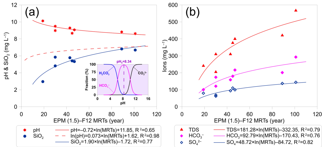
Figure 12. (a) pH and silica ( \text{SiO}_2 ) and (b) sulfate ( \text{SO}_4^{2-} ), bicarbonate ( \text{HCO}_3^- ), and total dissolved solids (TDS) vs. mean residence times (MRTs). The MRTs are from CFC-12 data using the EPM (1.5) model. The dashed red line in (a) is from Morgenstern et al. (2015).
