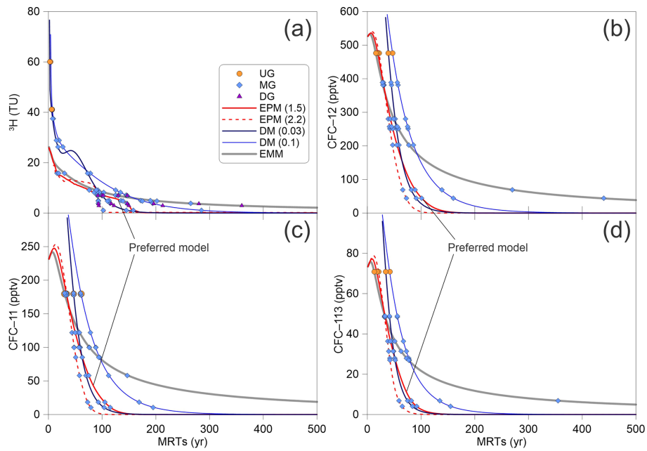
Figure 10. Tritium and CFCs (CFC-11, CFC-12, and CFC-113) output vs. mean residence times for different lumped parameter models estimated using Eqs. (2) to (5). The input ^3\text{H} activity and CFCs concentration are using the estimated ^3\text{H} activity in precipitation in Urumqi station (Fig. 4) and the Northern Hemisphere atmospheric mixing ratio (Fig. 3), respectively.
