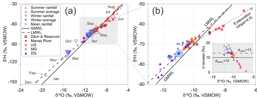
Figure 5. (a) Plot of stable isotopes of surface water and groundwater from the mountain to the oasis plain compared to the global meteoric water line (GMWL; Craig, 1961) and the local meteoric water line (LMWL, rainfall in Urumqi station of IAEA networks during 1986 and 2003; data are available at https://www.iaea.org , last access: 27 January 2016). The size of the hollow triangles stands for the relative amount of precipitation. “Mean rainfall” refers to the annual amount-weighted mean rainfall isotopic value. (b) Plot of \delta^2\text{H} vs. \delta^{18}\text{O} and inserted plot d excess vs. \delta^{18}\text{O} . UG: upstream groundwater, MG: midstream groundwater, DG: downstream groundwater.
