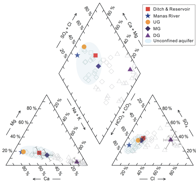
Figure 6. Piper diagram highlights the \text{HCO}_3\text{--SO}_4\text{--Na} type of waters. The coloured symbols represent the mean values calculated from the hydrochemistry data (light grey hollow symbols) reported by Ma et al. (2018). The error bars are shown in the cation and anion diagrams.
