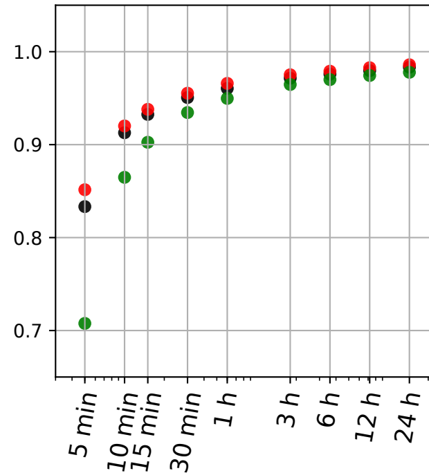
(a) Nugget
