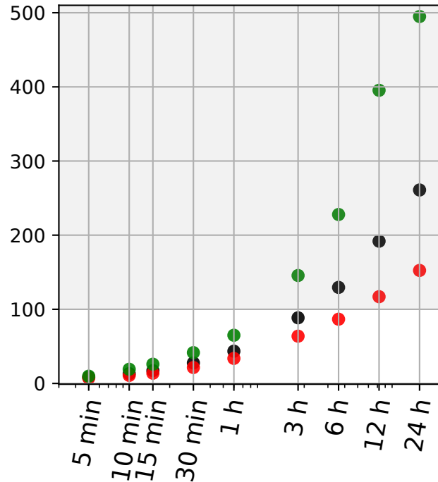
(b) Correlation distance [km]
