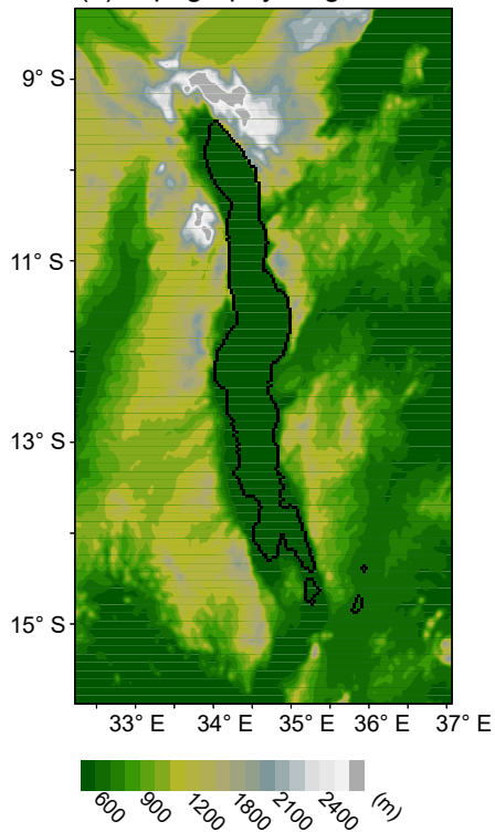
(a) Topography height
