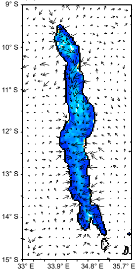
(a) WRF-CTL
