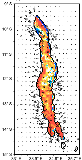
(f) Difference
