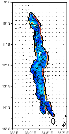
(c) Difference
