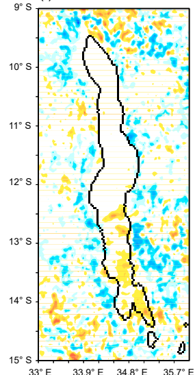
(f) Difference
