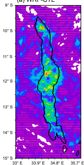
(a) WRF-CTL
