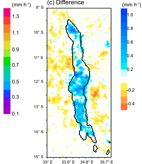
(c) Difference
