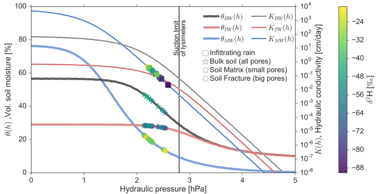
5 Figure S 2 Water retention curves ( \theta(h) , thick lines) and hydraulic conductivity ( K(h) , thin lines) for bulk soil (grey), small soil pores holding tightly bound water (Soil matrix, red), and big pores routing mobile water (Soil Fracture, blue). The color code of squares represent monthly weighted averages of rainfall stable isotopic composition (same as squares in Figure 3b), colors of stars and circles show observed isotopic compositions for each day of sampling of bulk and mobile soil waters, respectively (same as BW and MW in Figure 1 and 2), and colors of the pentagons are derived isotopic compositions of tightly bound water (TW in Figure 2). The distinction of the water retention and hydraulic conductivity curves between soil matrix and fractures were made based on the dual-porosity approach proposed by Gerke & van Genuchten (Gerke and van Genuchten, 1993) and the values for the van Genuchten parameter (van Genuchten, 1980) were based on pedotransfer functions (Schaap et al., 2001) (values shown in Table S3). 10
