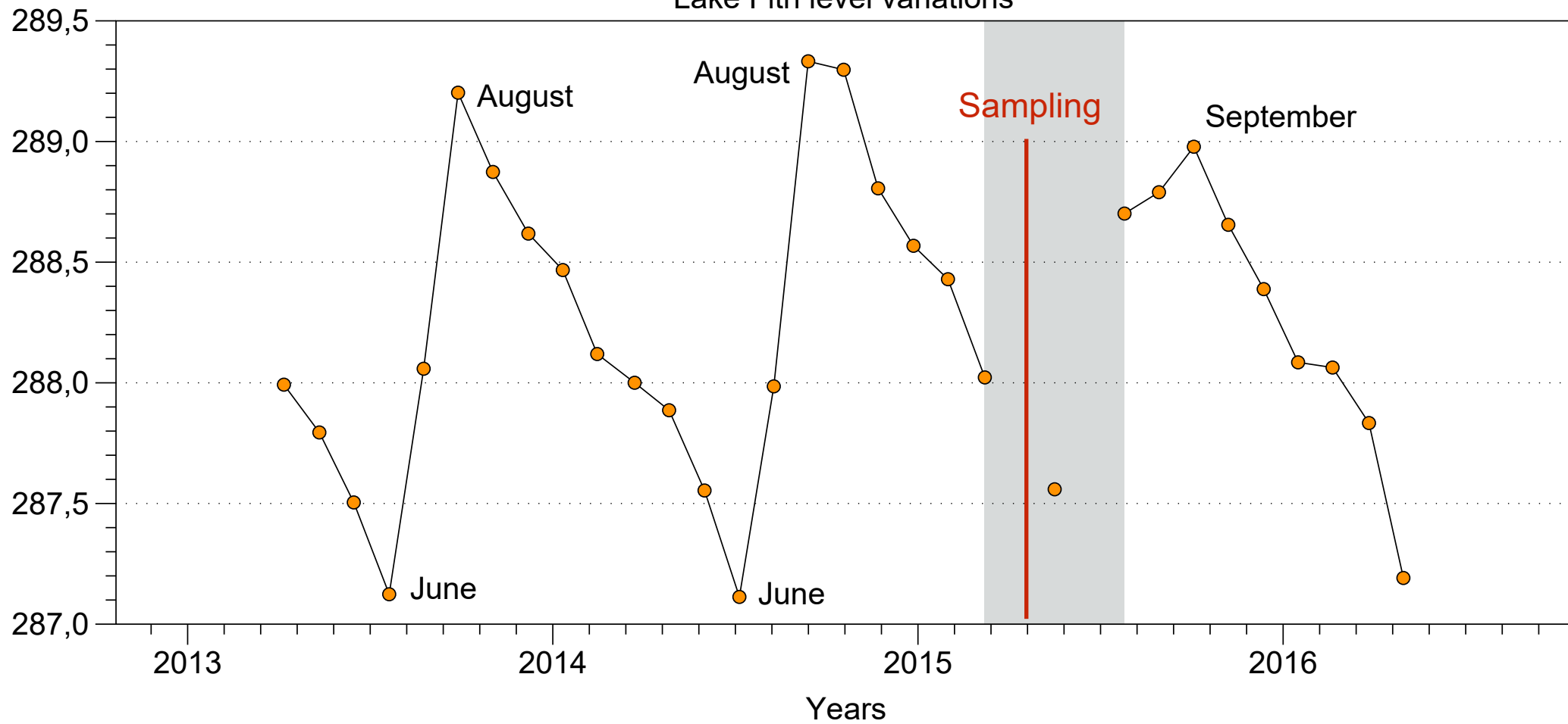
Lake Fitri level variations
