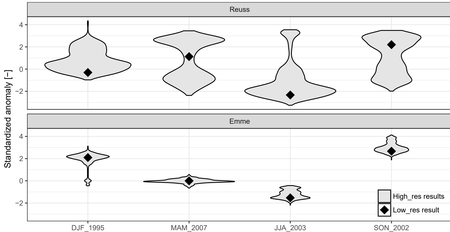
(a) Generated runoff anomalies
