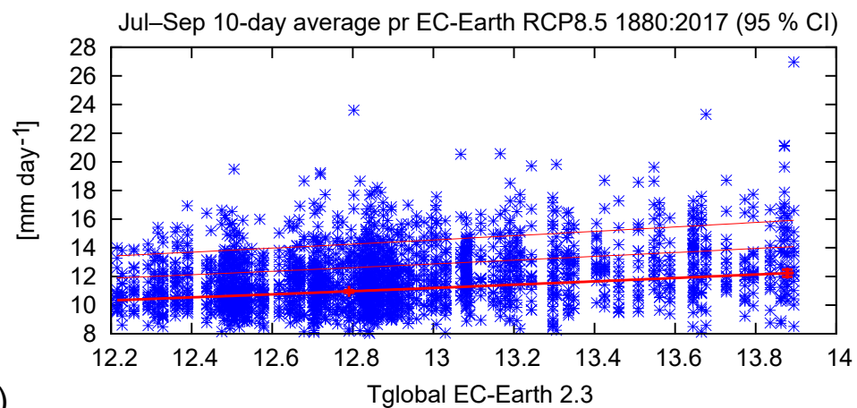
Jul–Sep 10-day average pr EC-Earth RCP8.5 1880:2017 (95 % CI)
