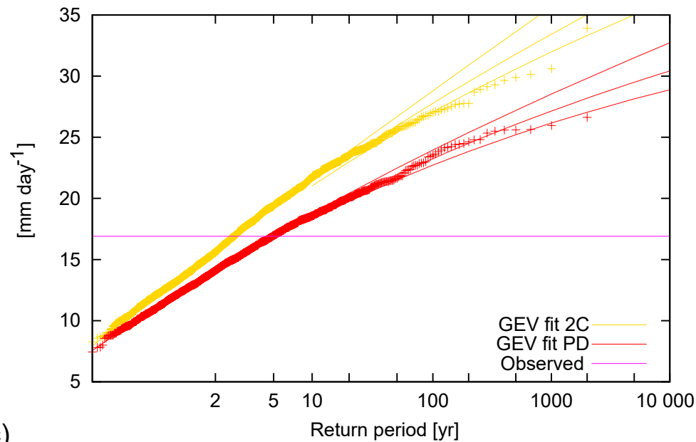
Jul–Sep 10-day average pr EC-Earth PD and 2C (95 % CI)
