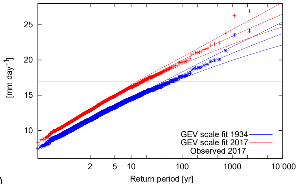
Jul–Sep 10-day average pr EC-Earth RCP8.5 1880:2017 (95 % CI)
