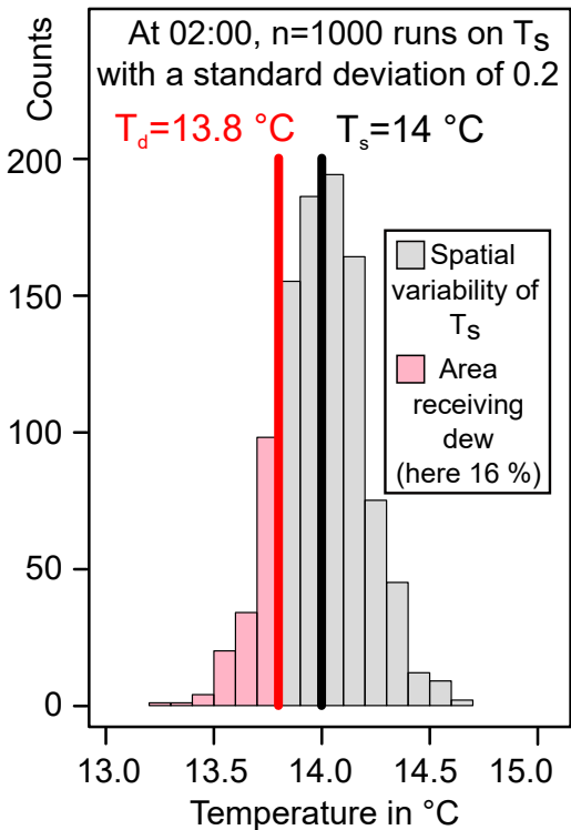
(a) Monte Carlo example
