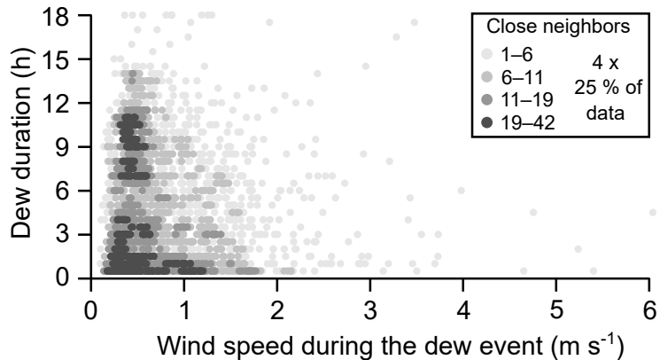
(d) Forests and grasslands, density plot (1918 dewy nights)
