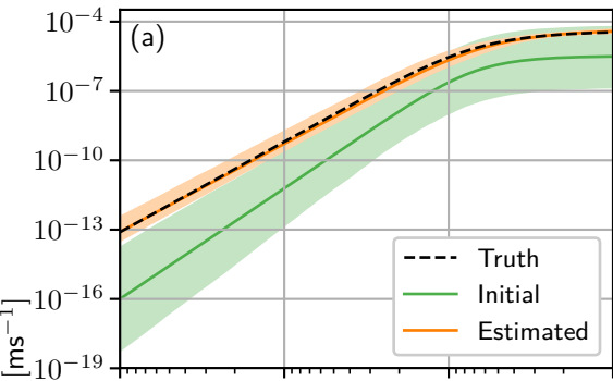
Conductivity - layer 1, 10 %
