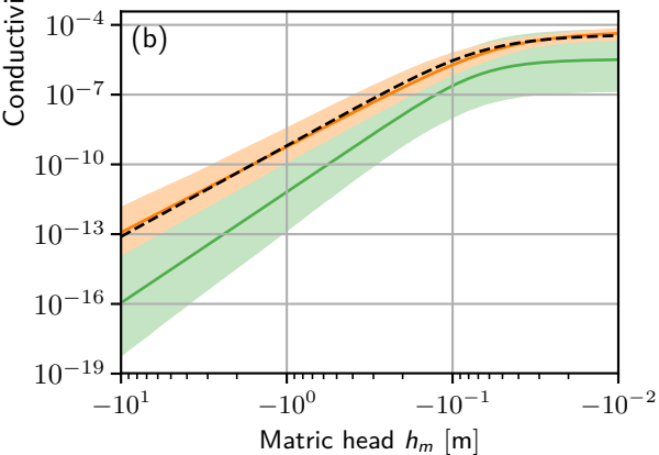
Conductivity - layer 1, 20 %
