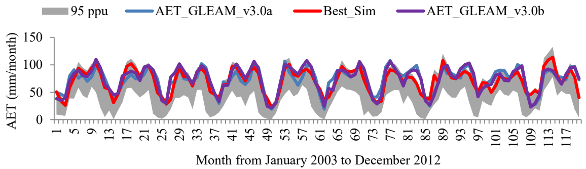
AET subbasin 34 (Iseyin weather station, Ogun River basin)
