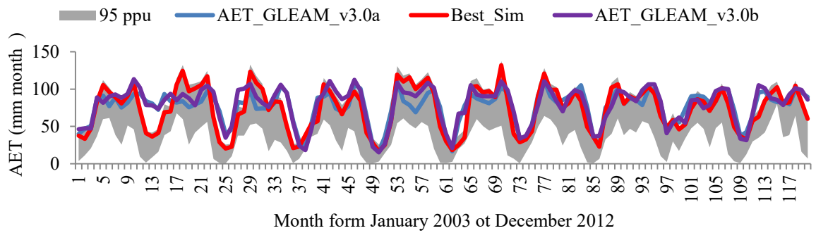
AET subbasin 53 (Abeokuta weather station, Ogun River basin)
