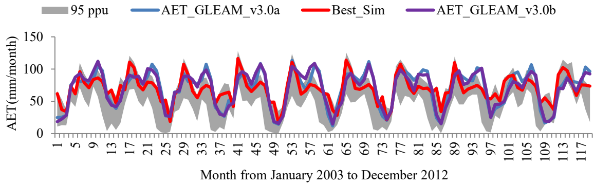
AET subbasin 5 (Saki weather station, Ogun River basin)
