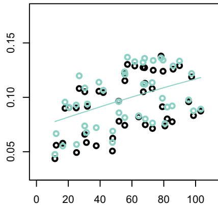
Fisher copula
