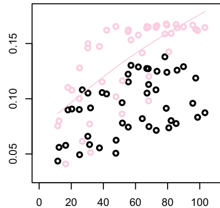
Gaussian m-s
