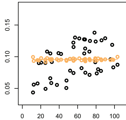
Brown-Resnick m-s
