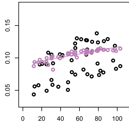
Brown-Resnick m-s
