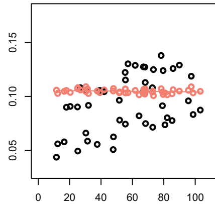
Gaussian m-s
