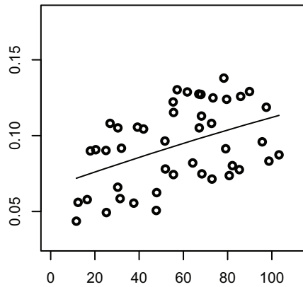
Fisher copula
