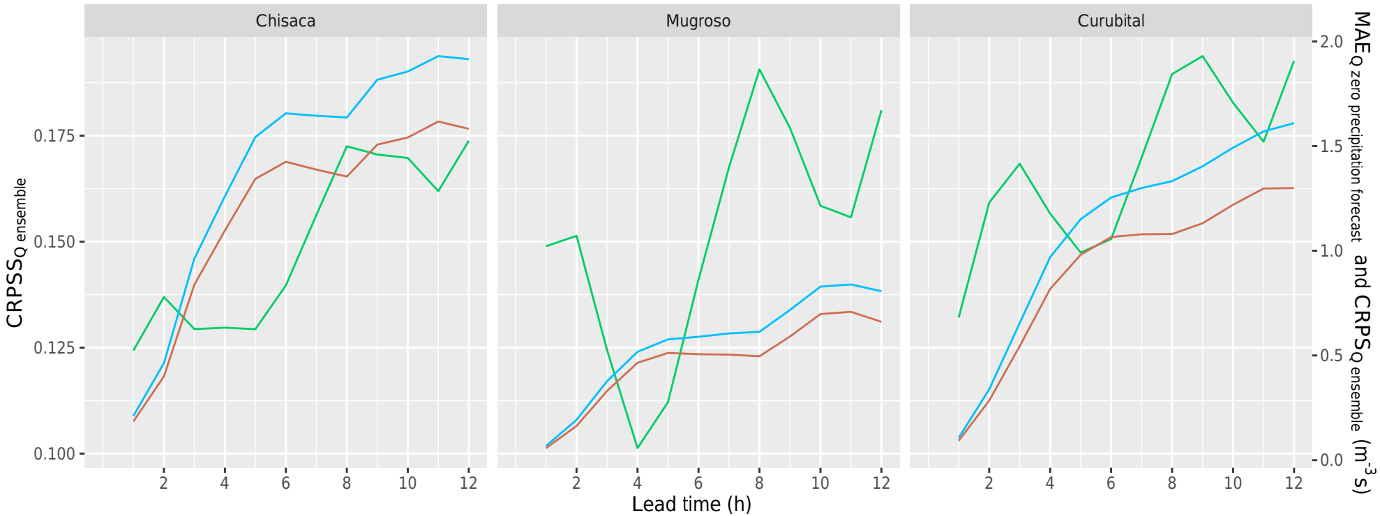
— MAE Q zero precipitation forecast — CRPS Q ensemble — CRPSS Q ensemble
