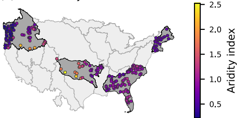
(b) Basin aridity
