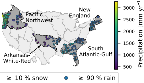
(a) Mean annual precipitation
