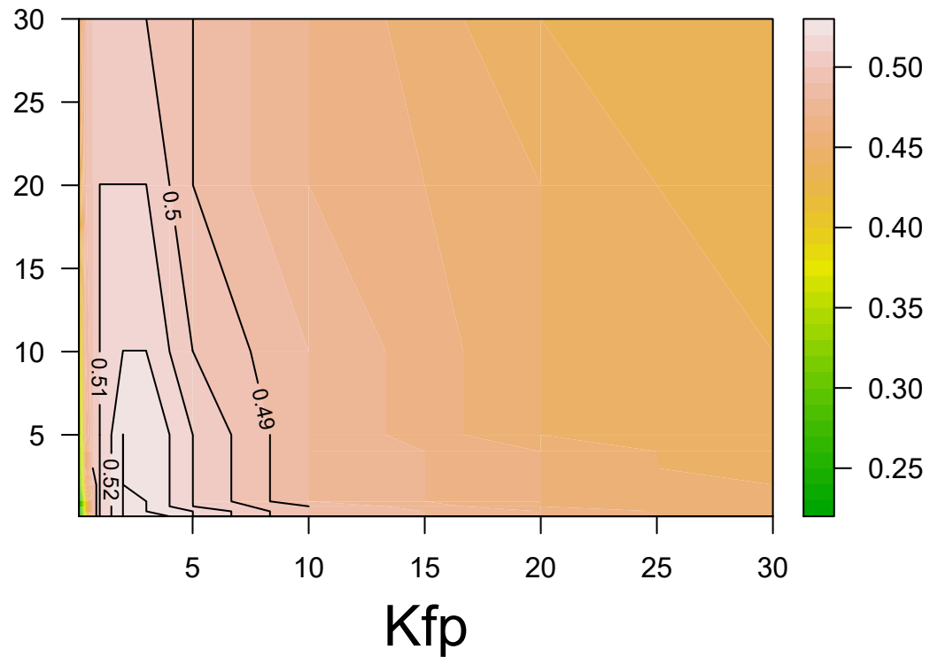
(b) CSI (max = 0.53)
