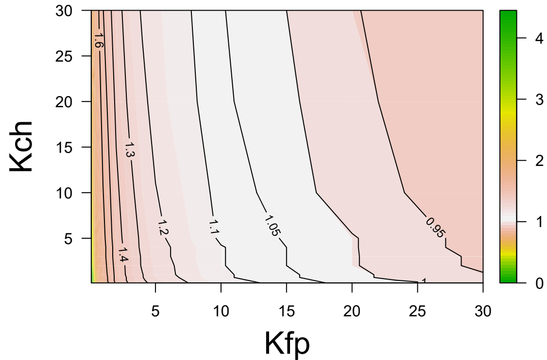
(a) BIAS (best = 1)
