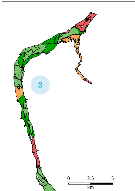
(a) BIAS
