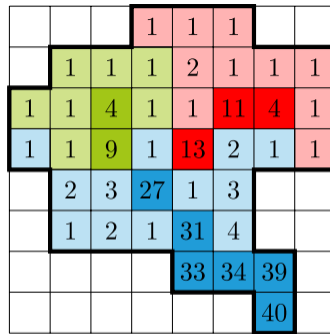
(c) Drainage area and sub-catchments
