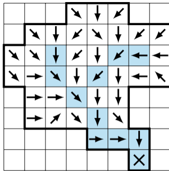
(b) Drainage direction
