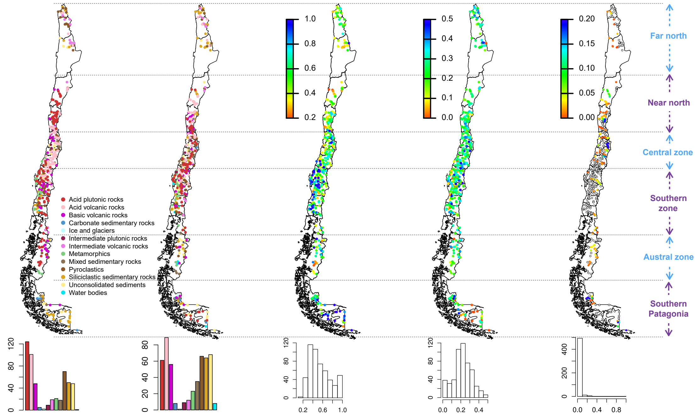
(a) Most common class (b) Second most common class (c) Fractional area of most common class [-] (d) Fractional area of second most common class [-] (e) Fractional area of carbonate sedimentary rocks [-]
