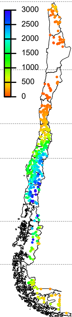
(b) Mean annual precipitation (mm)
