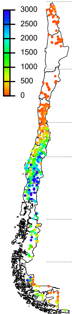
(a) Mean annual runoff (mm)
