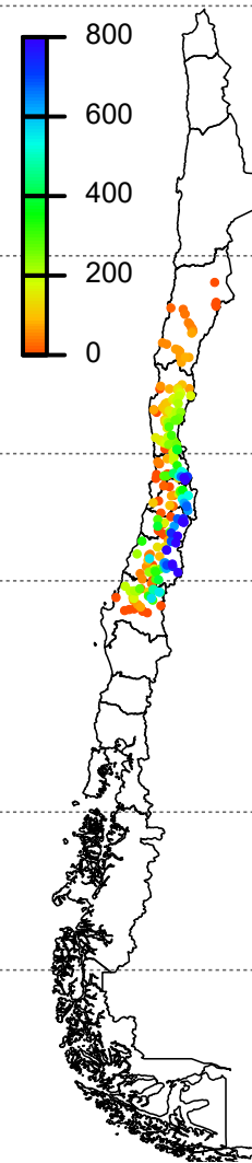
(e) Mean annual maximum SWE (mm)
