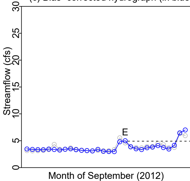
(c) Bias-corrected hydrograph (in blue)
