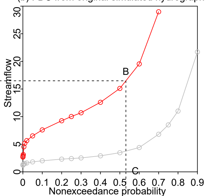
(b) FDC from original simulated hydrograph
