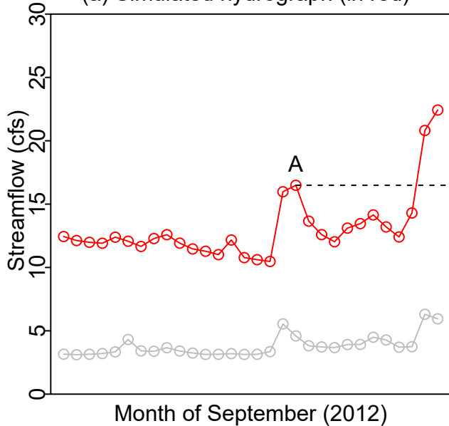
(a) Simulated hydrograph (in red)
