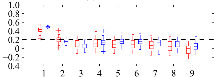
(c) UHRB-SON
