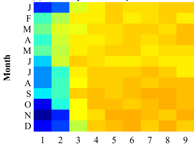
(a) UHRB-predictability
