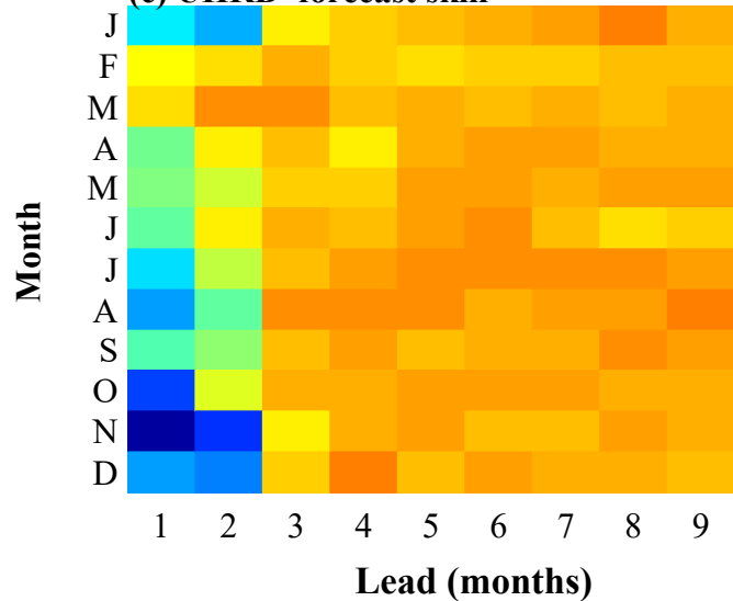
(c) UHRB-forecast skill
