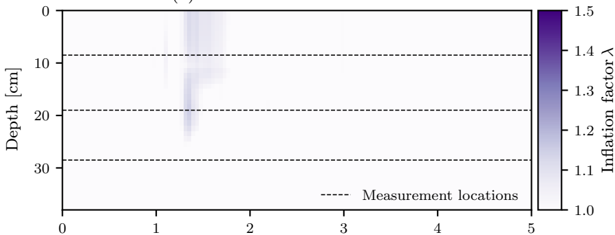
(c) Inflation with closed-eye EnKF
