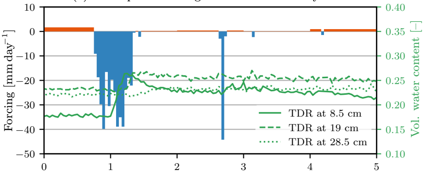
(b) Inflation with standard EnKF
