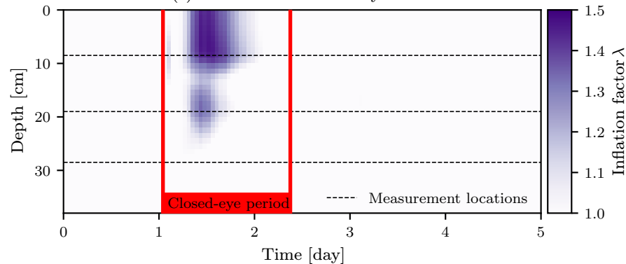
(c) Inflation with closed-eye EnKF
