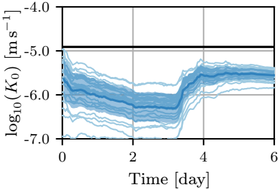
(a) Sat. hydraulic conductivity
