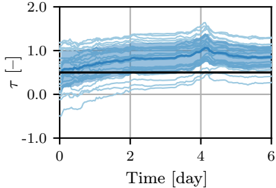
(b) Tortuosity \tau
