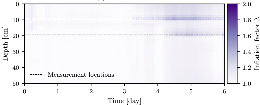
(b) Sat. hydraulic conductivity
