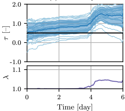
(c) Tortuosity \tau
