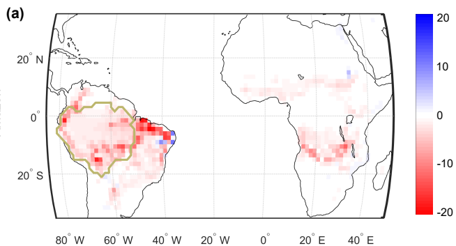
Precipitation source change \Delta P_{\text{tracked,basin}}
