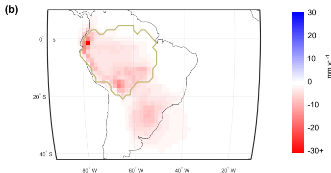
Evaporation sink change \Delta E_{\text{tracked,basin}}
