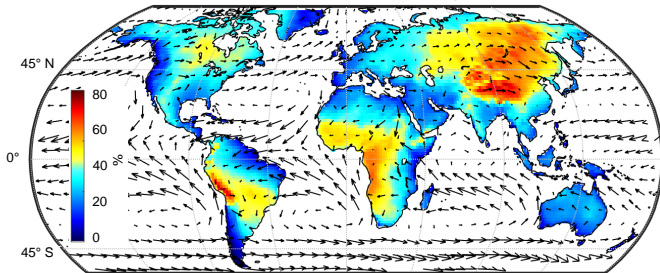
Continental precipitation recycling ratio
