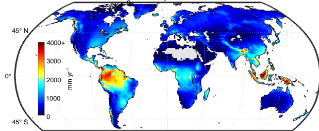
River flows at outlet
