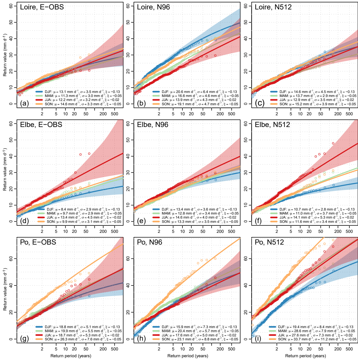
Figure 4. Fitted GEV distributions for (a–c) Loire, (d–f) Elbe, and (g–i) Po river basins, and for (a, d, g) E-OBS observed precipitation, (b, e, h) the N96 model, and (c, f, i) the N512 model. 95% resampling confidence intervals are shown as shaded areas for winter (DJF) and summer (JJA). Block maxima (circles) are shown at return periods \frac{m+1}{m+1-i} , where m is the number of these maxima, i.e. here the number of years \times ensemble members, and i = 1, \dots, m is their rank. Results for N216 are generally between those for N96 and N512 (not shown). The three basins are indicated in Fig. 5a and d.
