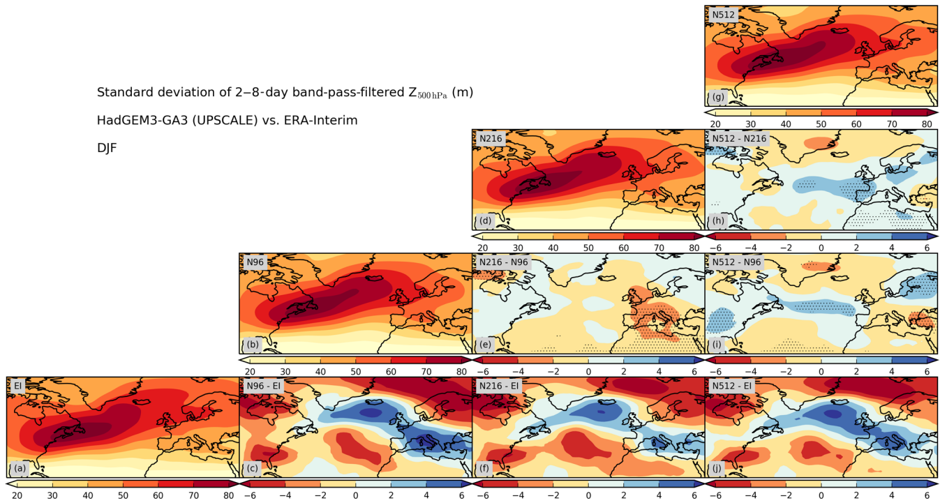
Figure 7. Standard deviation of 2–8-day band-pass-filtered 500 hPa geopotential height (m). (a) ERA-Interim reanalysis, (b, d, g) model (HadGEM3-GA3) at resolutions N96, N216, and N512, (c, f, j) model biases with respect to ERA-Interim, and (e, h, i) differences between model resolutions. Stippling shows statistically significant differences.
