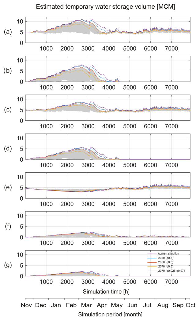
Figure 8. Impacts of the median climate scenarios ( q0.5 ) for years 2030, 2050 and 2070 as well as the uncertain climate scenarios (1000 random sampled combinations) for 2070 on (a) the simulated water storage of the whole catchment, (b) the simulated snow storage of the whole catchment, (c) the simulated water storage of the karst area, (d) the simulated snow storage of the karst area, (e) the simulated water storage of the karst aquifer, (f) the simulated water storage of the non-karst area and (g) the simulated snow storage of the non-karst area.
