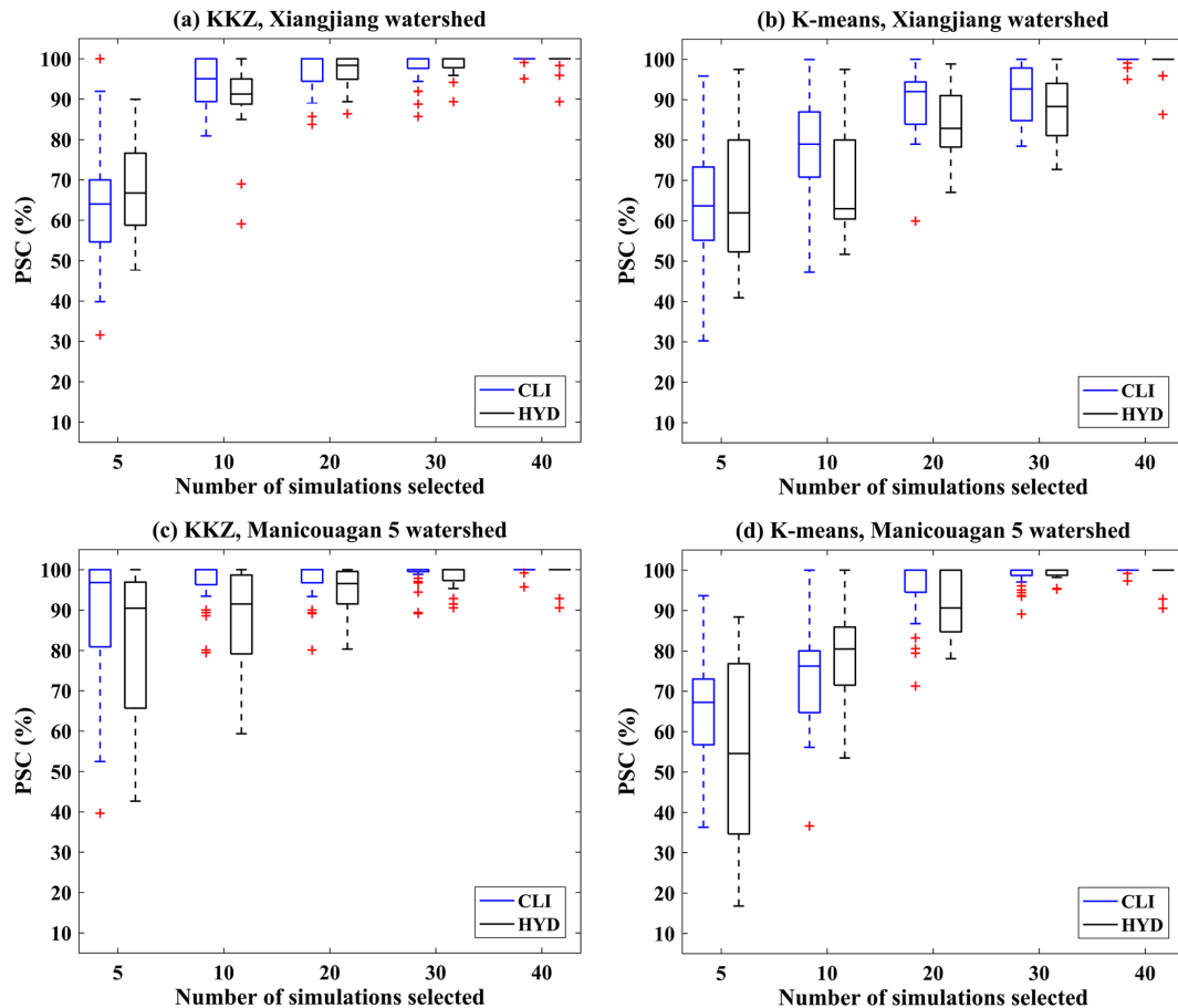
Figure 6. Boxplots of the PSCs of 31 climate variables (CLI) and 17 hydrological variables (HYD) when selecting different numbers of climate simulations over two watersheds using the KKZ method and K means clustering.
