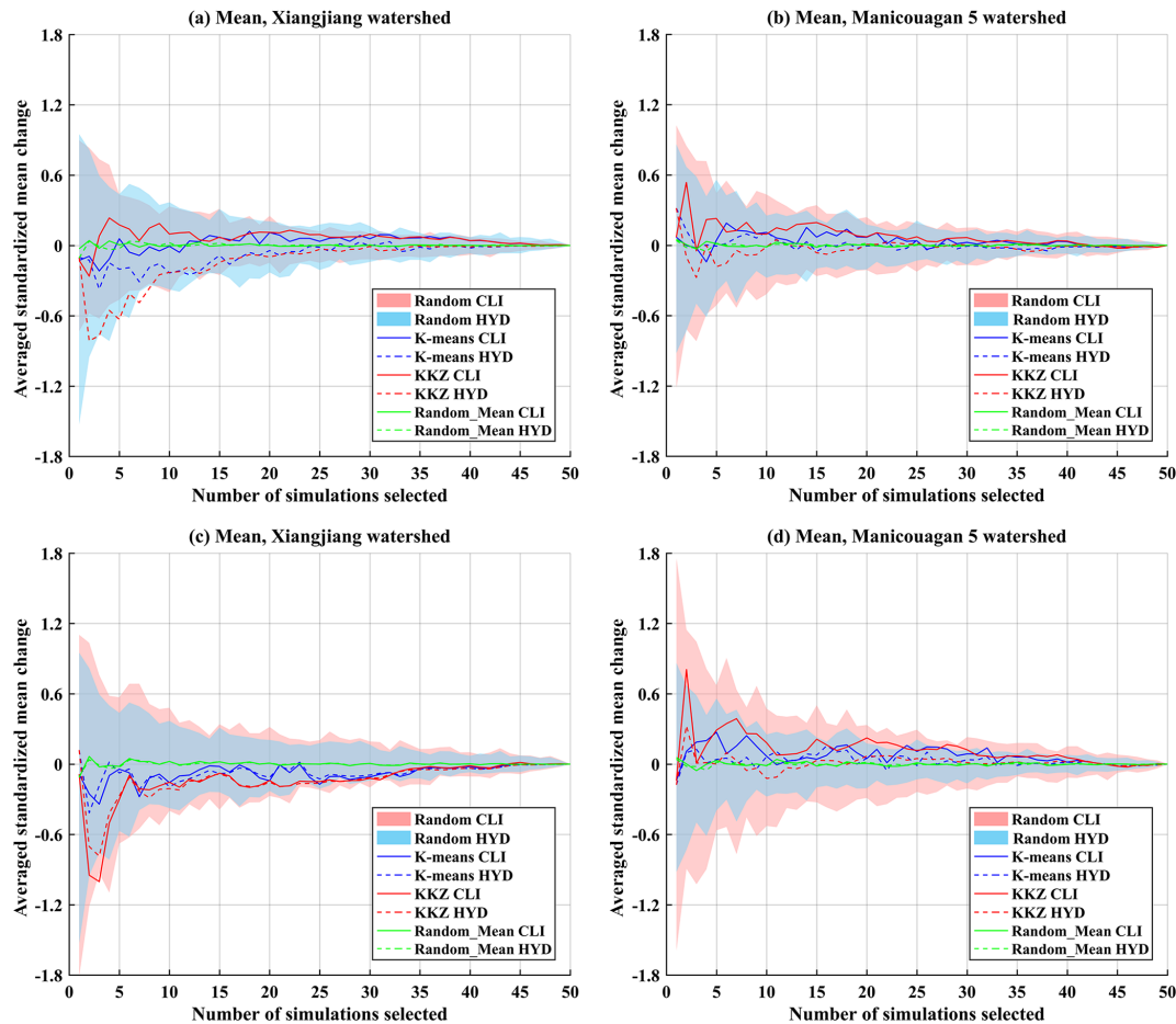
Figure 9. Averaged standardized mean change in climate (CLI) and hydrological (HYD) variables of subsets selected by three selection methods ( K means, KKZ and random selection) over the Xiangjiang and Manicouagan 5 watersheds when temperature variables are (a, b) included or (c, d) excluded in the process of selection. The pink and blue panels are the envelopes resulting from 100 random selections.
