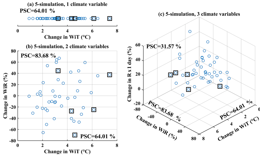
Figure 2. Examples of PSCs when selecting five climate simulations over the Xiangjiang watershed using the KKZ method. The PSCs of each variable are presented beside the corresponding axes.
