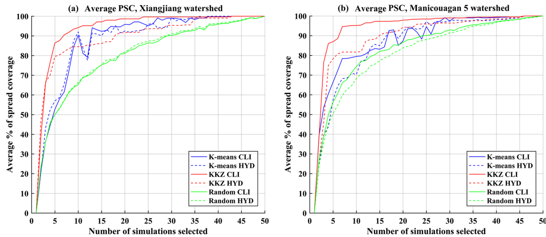
Figure 10. The average PSC for three different selection methods ( K means, KKZ and random selection) over two watersheds when using QM methods (temperature variables are excluded in the Xiangjiang watershed, while they are included in the Manicouagan 5 watershed).
