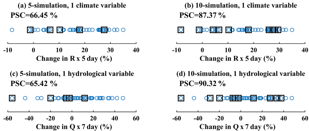
Figure 4. Examples of the transferability of climate uncertainty to hydrological impacts based on one variable when selecting (a, c) 5 and (b, d) 10 climate simulations over the Xiangjiang watershed using the KKZ method. The PSCs of each variable are presented in the top left corner.
