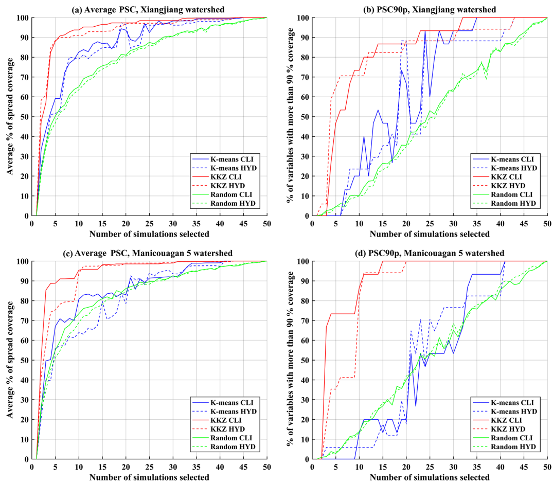
Figure 8. The (a, c) average PSC and (b, d) PSC90p for three different selection methods ( K means, KKZ, and random selection) over two watersheds when temperature variables are excluded in the process of simulation selection (CLI: climate variables; HYD: hydrological variables).
