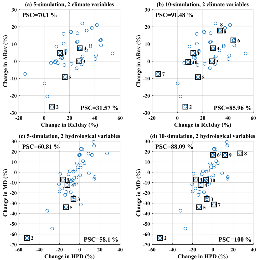
Figure 5. Examples of the transferability of climate uncertainty to hydrological impacts based on two variables when selecting (a, c) 5 and (b, d) 10 climate simulations over the Xiangjiang watershed using the KKZ method. The PSCs of each variable are presented beside the corresponding axes.
