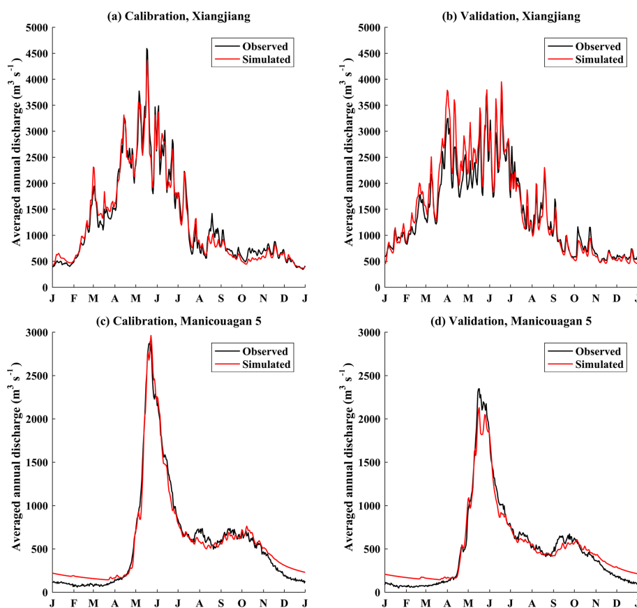
Figure 3. Observed and simulated mean hydrographs for (a, c) calibration and (b, d) validation periods over the (a, b) Xiangjiang and (c, d) Manicouagan 5 watersheds.
